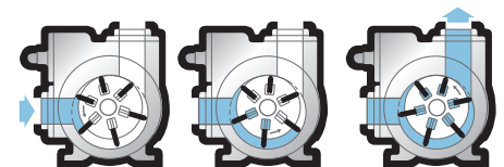
How Blackmer's sliding vane action works
